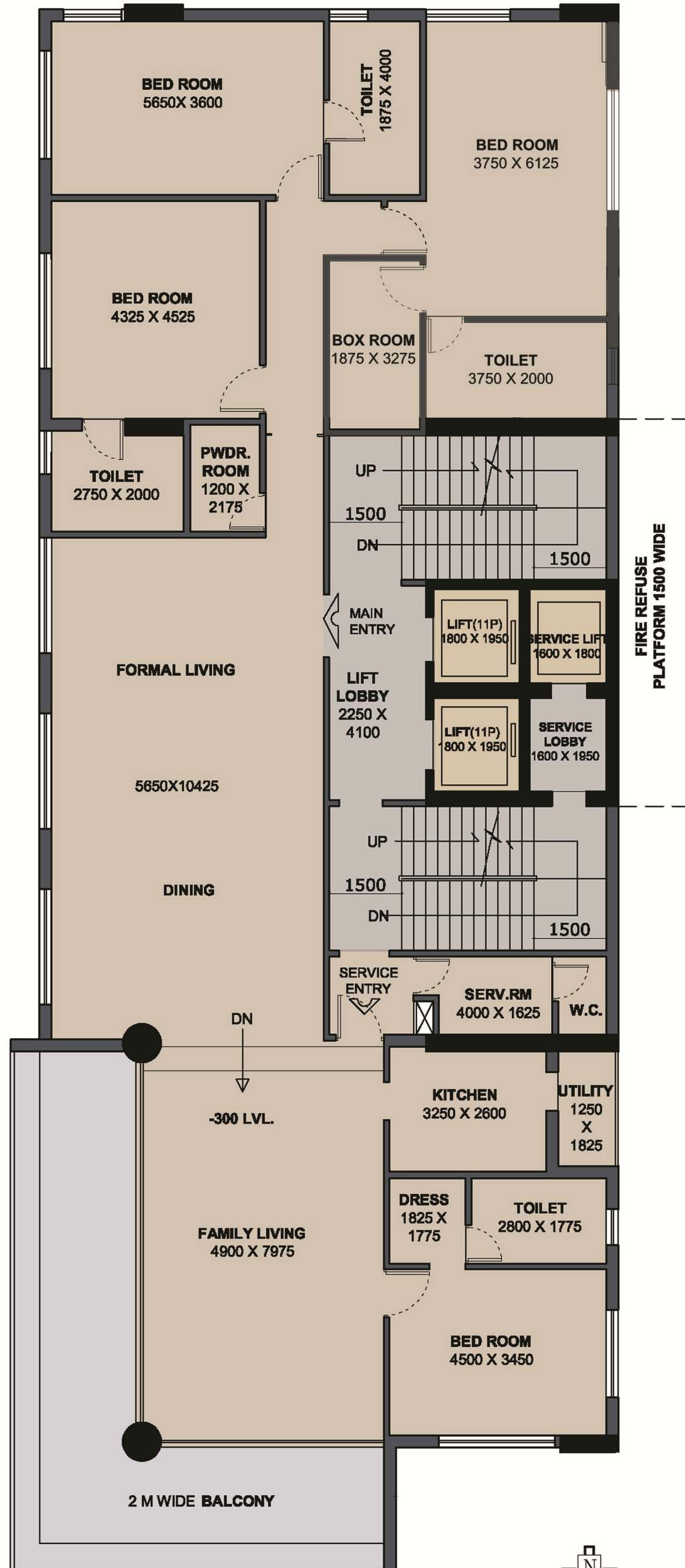
TYPICAL FLOOR PLAN (FIRST TO FIFTH FLOOR)
