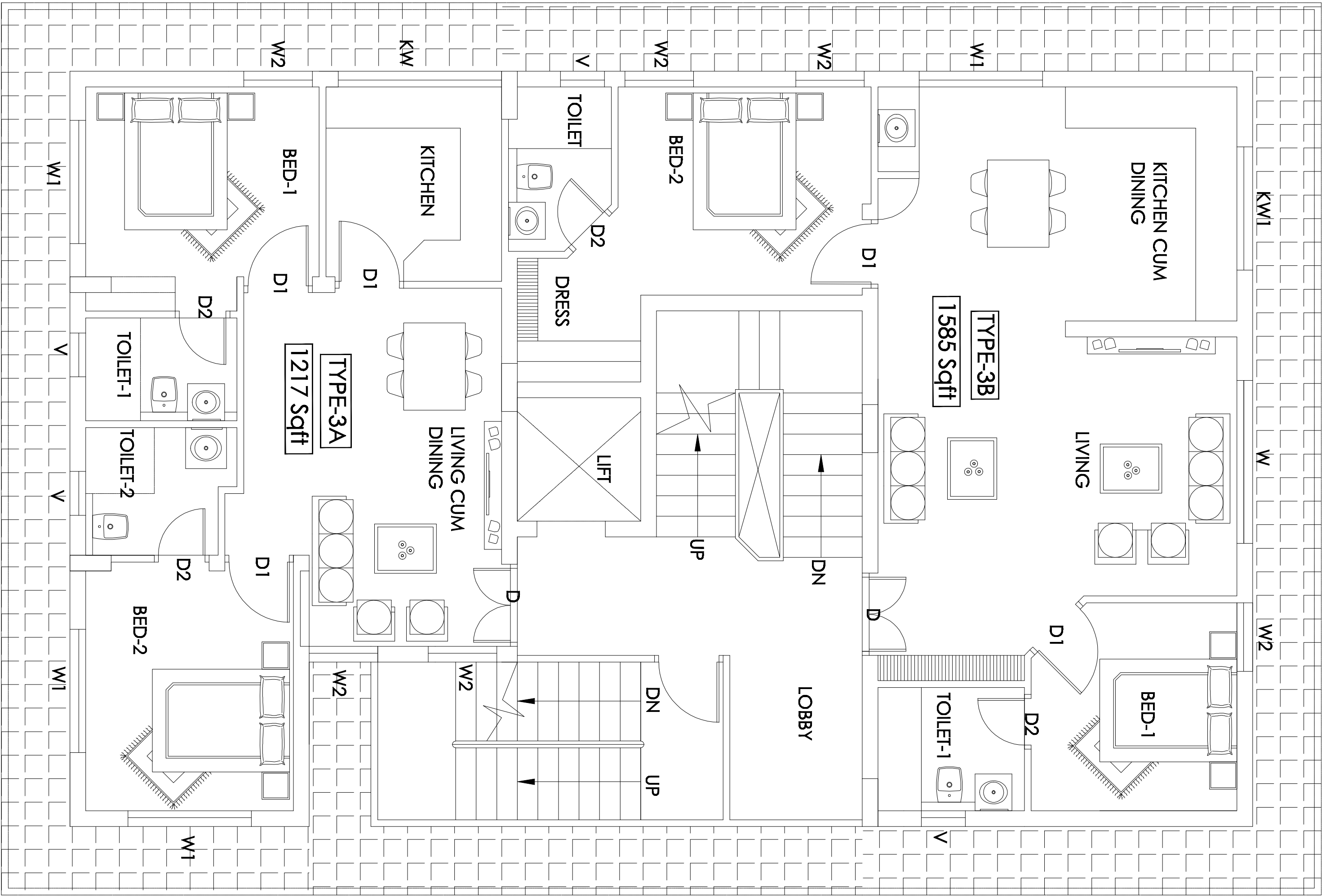
3rd floor plan
